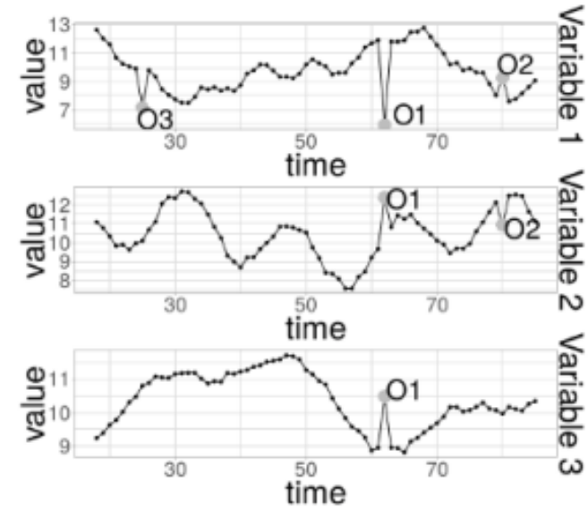
(b) Multivariate time series.
