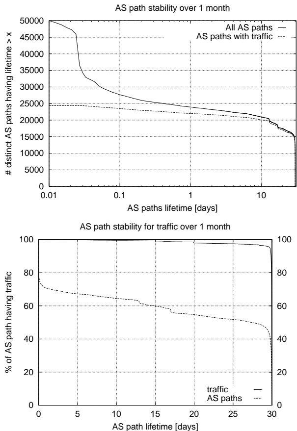
Figure 2: Stability of AS paths: without traffic (top) and with traffic (bottom).
