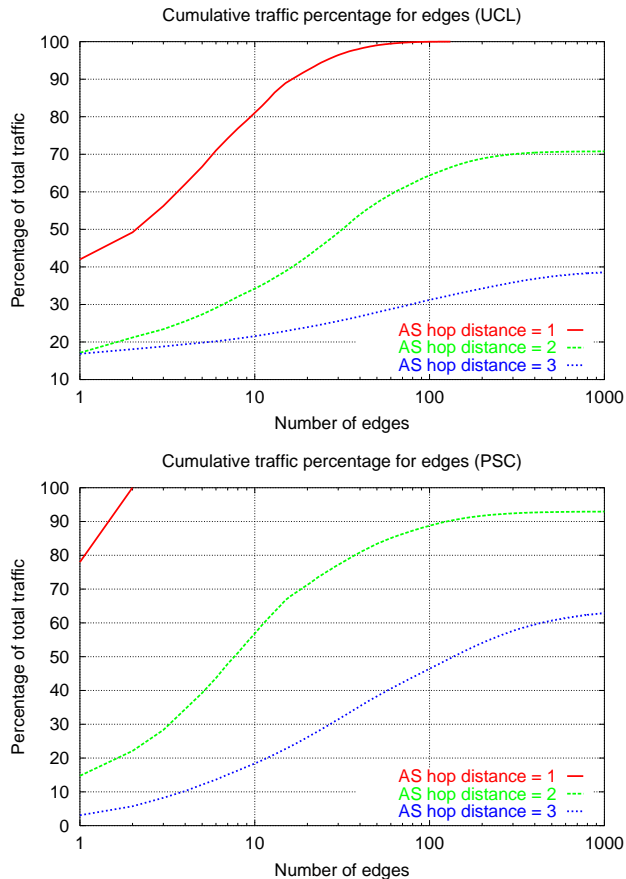
Figure 3: Cumulative traffic captured by edges : UCL (top) PSC (bottom).
