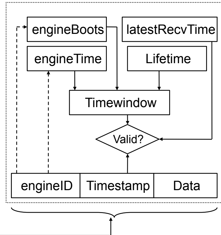
Receiver
